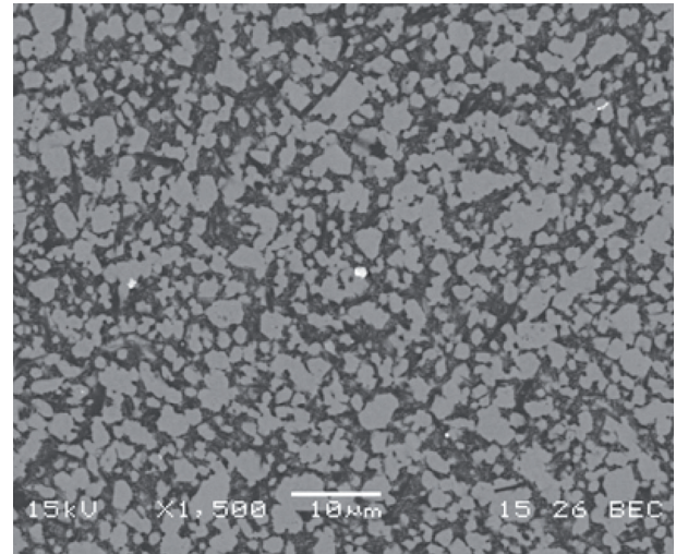
SEM microstructure of EDM-Si 3 N 4
